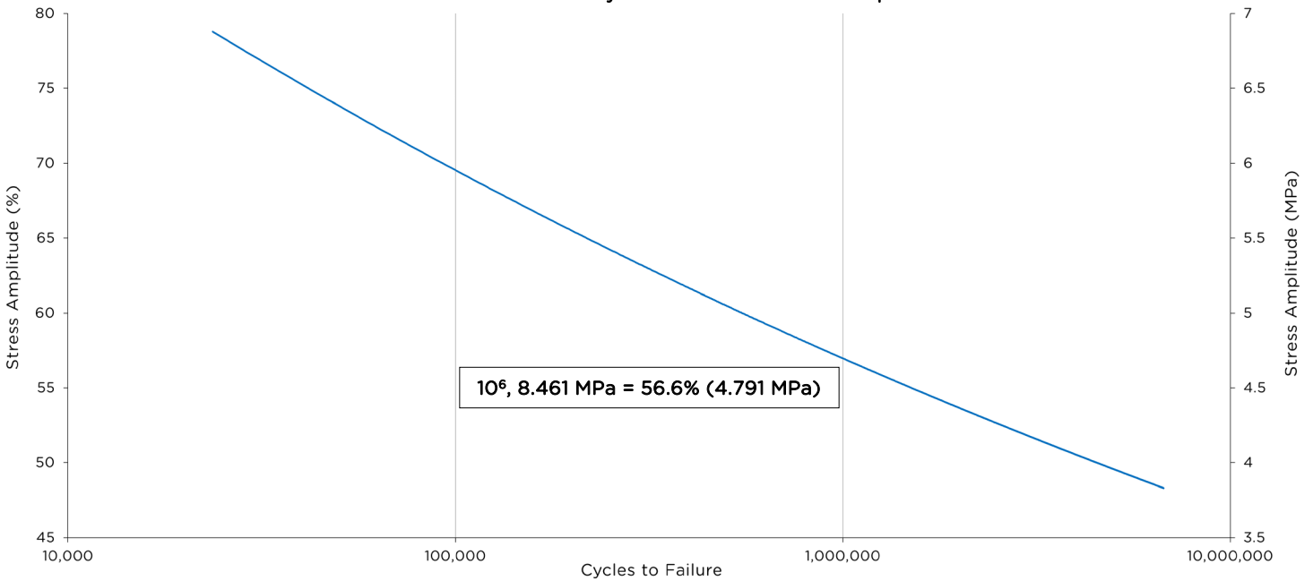
ISO 9664 - Belzona 7311 Cycles to Failure vs. Stress Amplitude
